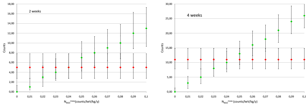
Figure 8.26: Average number of counts and 68% Confidence Level limit for the array of four 5x5x5 cm 3 BGO for 2 weeks (left) and 4 weeks (right) of live time. The number of events expected N_{BGO}^{exp} in the case of a surface contaminations equal to that of the TTT is shown in red while in green the one corresponding to a counting rate less than 0.1 counts/keV/kg/y.
