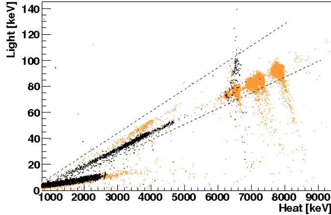
Figure 8.18: Scatter plot of light vs. heat recorded with the Huge ZnSe crystal in two different runs. In run I (colored points) the B alpha source was mounted on the bottom side of the crystal, opposite to the LD. In run II (black points) source B was moved on the side of the crystal and in its place was mounted source A. The dotted lines identify the opening of the alpha band on a wide angle, due to the variation of the \text{QF}_\alpha upon source position.
