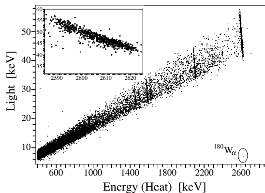
Figure 8.9: Scatter plot light vs. heat obtained in a 96 h calibration using an external ^{232}\text{Th} source. In the inset the highlight of the ^{208}\text{Tl} line. In the circle two events due to the internal \alpha -decay of ^{180}\text{W} . The energy spectrum below 400 keV is completely dominated by the ^{113}\text{Cd} \beta -decay, with a rate close to 0.4 Hz.
