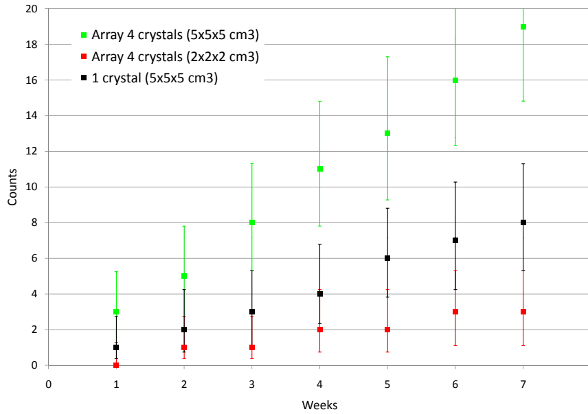
Figure 8.25: Number of expected counts in an energy region of 1 MeV as function of weeks for an array of four 2x2x2 cm 3 BGO crystals (red), a single 5x5x5 cm 3 BGO crystal (black) and an array of four 5x5x5 cm 3 BGO crystals (green).
