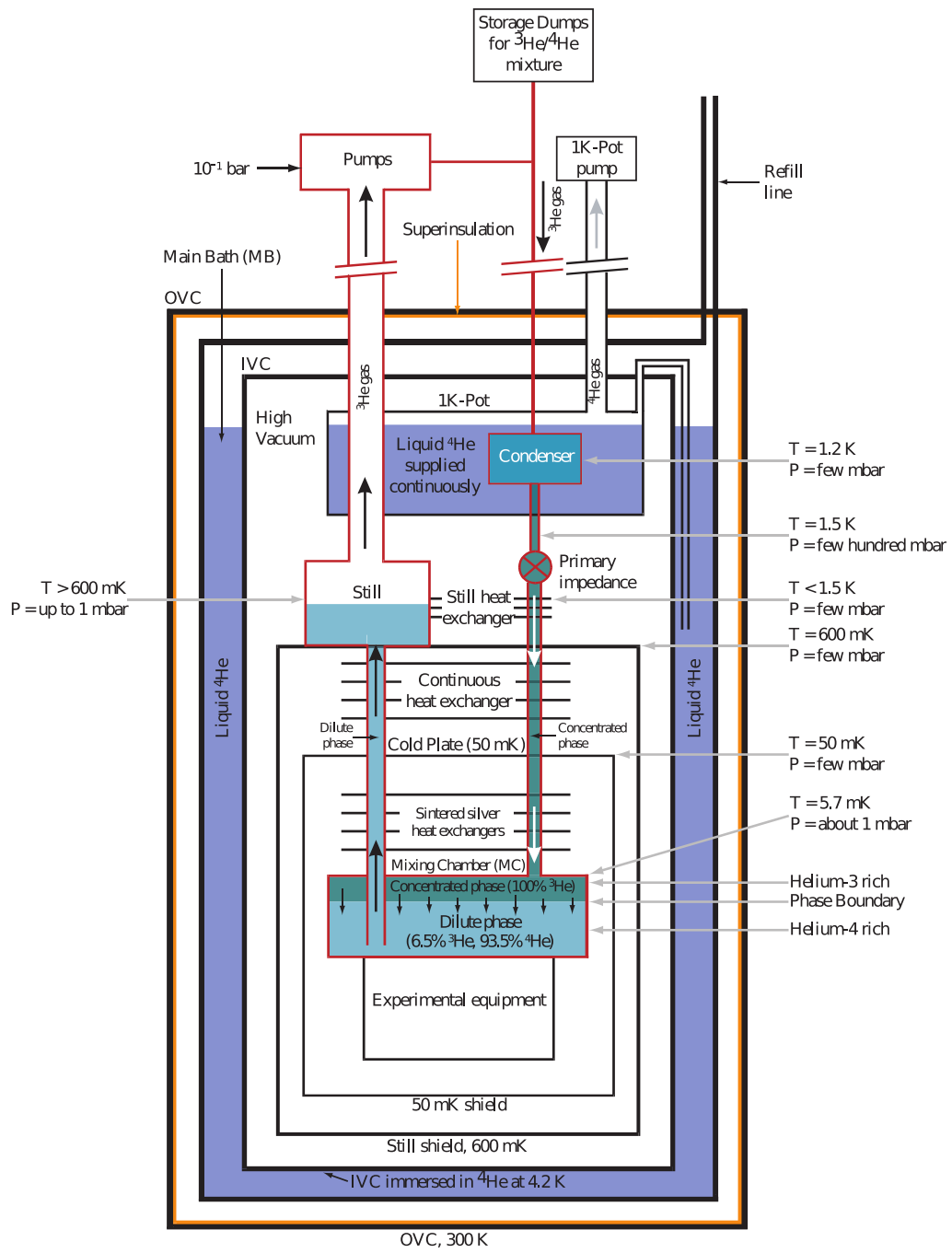
Figure 11.2: Schematic diagram of a conventional ^3\text{He}/^4\text{He} dilution refrigerator.
