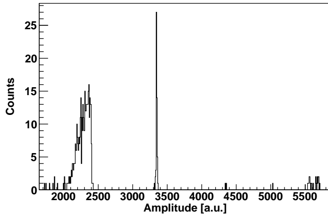
Figure 8.30: Spectrum of the \alpha region. It is possible to observe the broadened \alpha peak due to ^{147}\text{Sm} source and the sharp ^{209}\text{Bi} peak.
