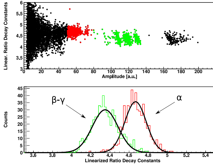
Figure 9.6: MgMoO 4 crystal: scatter plot of RDC^{lin} vs. Heat (top panel) and projection of 2-4 MeV events on the RDC^{lin} axis (bottom panel). In green events in the 2-4 MeV regions due to \beta/\gamma particles and in red those due to \alpha 's.
