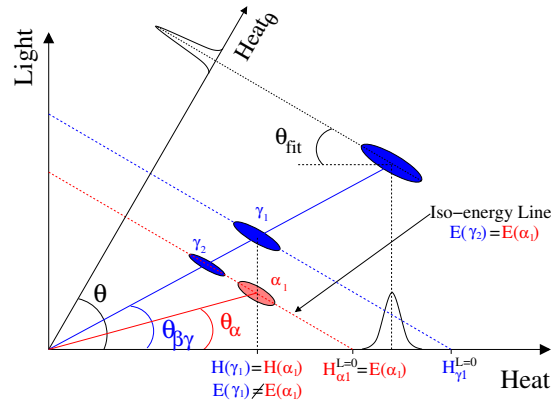
Figure 8.8: Light vs. heat scheme for the interpretation of the energy correction method. The blue (dark) spots represent the \gamma/\beta monoenergetic events, while the red (light) represents an \alpha .
