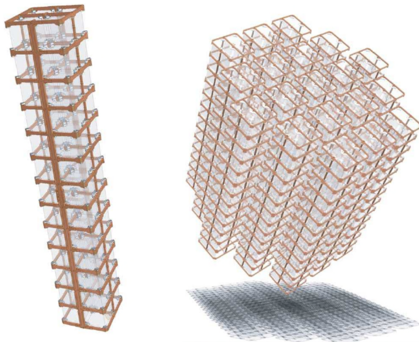
Figure 6.1: The CUORE modular structure. On top: two contiguous floors. Each frame is shared between two consecutive single modules. The copper columns join the two frames to fasten rigidly the crystals. Left on the bottom: A CUORE tower. 13 single modules are held together. Right on the bottom: the entire CUORE detector (cylindrical-shaped) built of 19 super modules.
