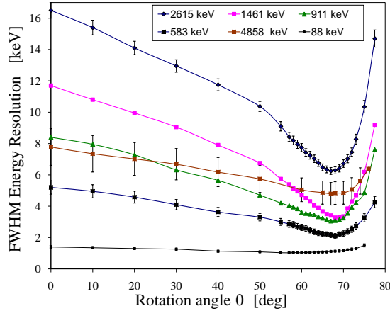
Figure 8.10: FWHM energy resolutions evaluated for different \theta angles. For each angle a spectrum is produced and the corresponding peaks are fitted. The curves through the data points are only to guide eyes. For two peaks the corresponding error on the FWHM is not plotted for better clarity.
