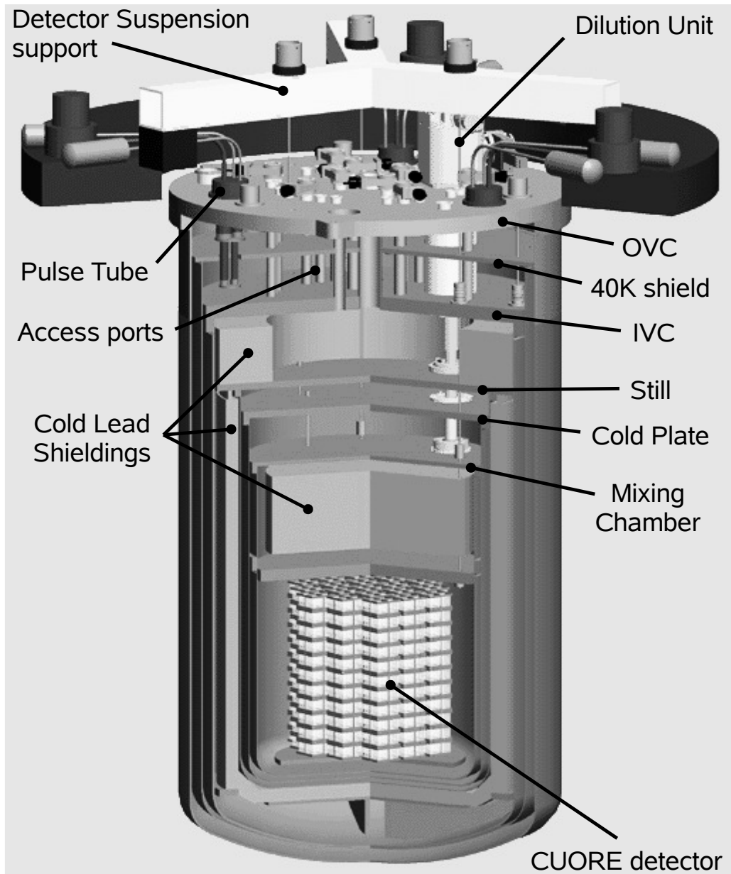
Figure 6.2: 3D view of the cryogenic apparatus.
