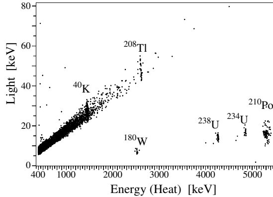
Figure 8.13: Scatter plot light vs. heat obtained in a 433 hours live time background measurement. Part of the ^{210}\text{Po} “bump” is characterized by smaller light emission. This could arise from a worse light collection efficiency, especially from the lateral part of the crystal. The energy scale of the \alpha is corrected according with what exposed in Sec. 8.3.1.
