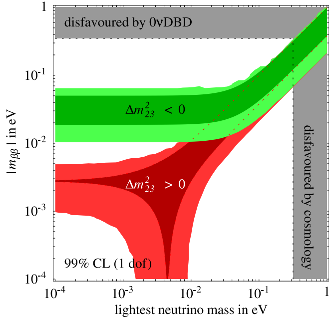
Figure 2.3: 99% C.L. expected ranges for the parameter |m_{\beta\beta}| as a function of lightest neutrino mass. \Delta m_{23}^2 > 0 corresponds to NH ( m_{lightest} = m_1 ), while \Delta m_{23}^2 < 0 corresponds to IH ( m_{lightest} = m_3 ). The darker regions show how the ranges would shrink if the present best-fit values of oscillation parameters were confirmed with negligible errors. [25]
