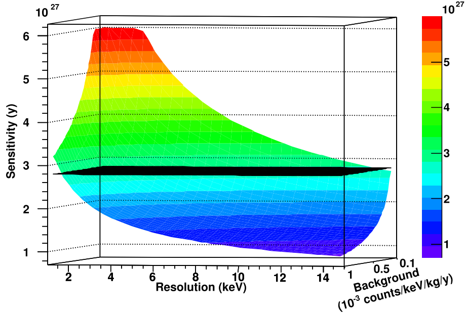
Figure 10.2: 0\nu DBD sensitivity as a function of energy resolution and background level with sensitivity cut-off due to the number of isotope candidates to 0\nu DBD, i.e. intersection of equation 10.1 and equation 10.2.
