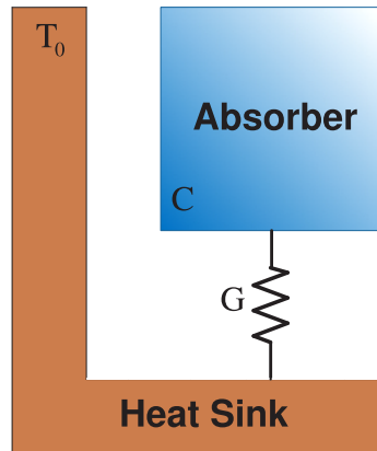
Figure 4.1: Simplified bolometer thermal model. The detector is modeled as a single object weakly coupled to the heat sink. The heat capacity C contains all the contribution of the elements which compose the detector. G describes the thermal conductance between the detector and the heat sink.
