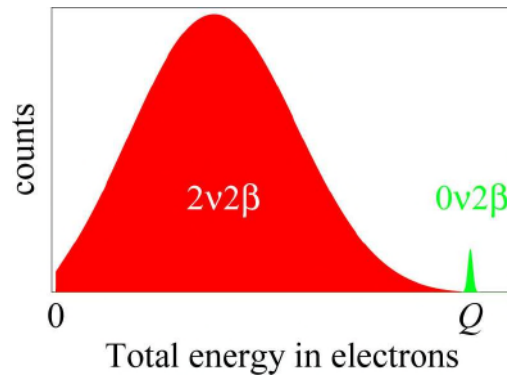
Figure 2.5: Experimental signature of 2\nu\text{DBD} and 0\nu\text{DBD}
