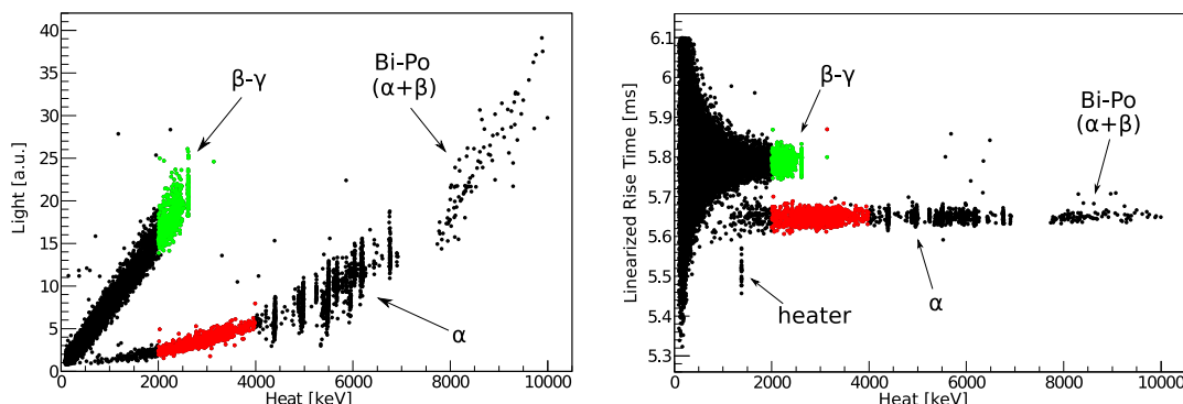
Figure 9.1: Scatter plot obtained with a CaMoO 4 crystal. Left panel: scatter plot of light vs. heat. The energy calibration is performed on the \gamma peaks. In red events in the 2-4 MeV region due to \alpha particles while in green events due to \beta/\gamma in the same region. Right panel: scatter plot of \tau_{rise}^{lin} vs. heat obtained for the same events. In green events in the 2-4 MeV regions due to \beta/\gamma particles and in red \alpha events.
