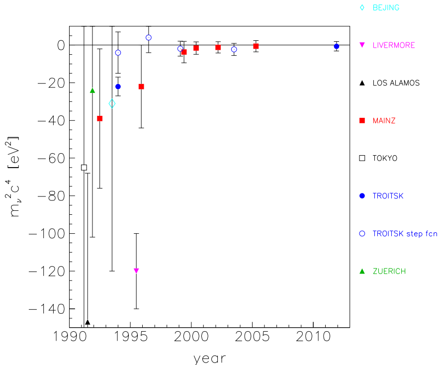
Figure 6: Historical trend of the m_{\nu_e}^2 measured with spectrometer using tritium (taken from [24]).
