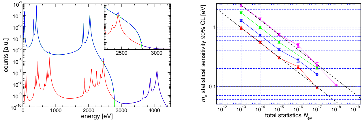
Figure 27: Calculated experimental ^{163}\text{Ho} EC calorimetric spectrum for Q = 2.8 keV, \Delta E = 2 eV, f_{pp} = 10^{-4} , and N_{ev} = 10^{14} (blue). The pile-up spectrum is the red curve (left). Monte Carlo estimated statistical sensitivity for \Delta E = 1 eV, \tau_R = 1 \mu\text{s} , and for f_{pp} = 10^{-3} , 10^{-4} , 10^{-5} , and 10^{-6} (from top to bottom). To two dashed lines correspond to (top) A_{EC} = 1000 Bq and N_{dey} \times t_M = 10^7 detector \times year and (bottom) A_{EC} = 1 Bq and N_{dey} \times t_M = 3 \times 10^9 detector \times year (right).
