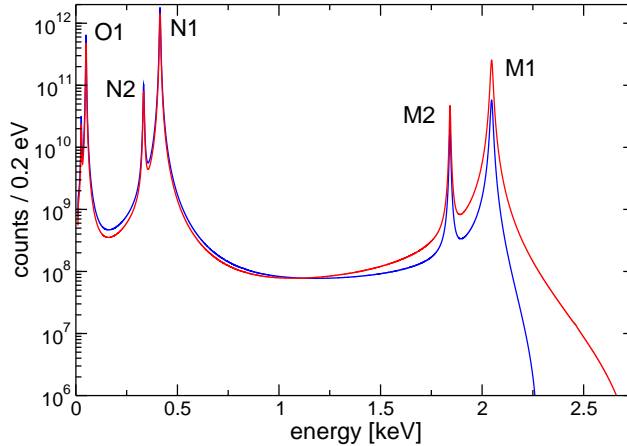
Figure 25: Calculated ^{163}\text{Ho} EC calorimetric spectrum for Q = 2.3 keV (blue) and Q = 2.8 keV (red), and for \Delta E = 2 eV and N_e v = 10^{14} .
