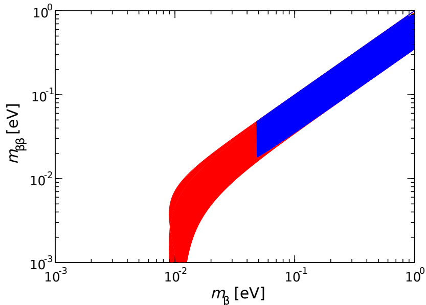
Figure 4: Relationship between the effective Majorana mass m_{\beta\beta} and the effective electron neutrino mass m_{\beta} for both IH (blue) and NH (red) mass schemes. The width of the bands is caused by the unknown Majorana phases.
