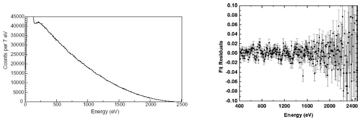
Figure 18: The MANU experiment final spectrum (left) and its fitting residuals showing the BEFS ripples (right) (from [108]).
