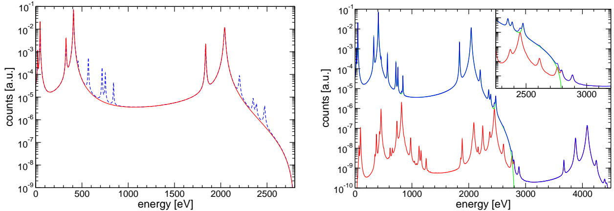
Figure 29: Predicted single and double holes calorimetric spectrum of the EC decay of {}^{163}\text{Ho} with Q = 2.8 keV (left). The experimental spectrum analogous to the one in Fig. 27 with double hole transitions included (right).
