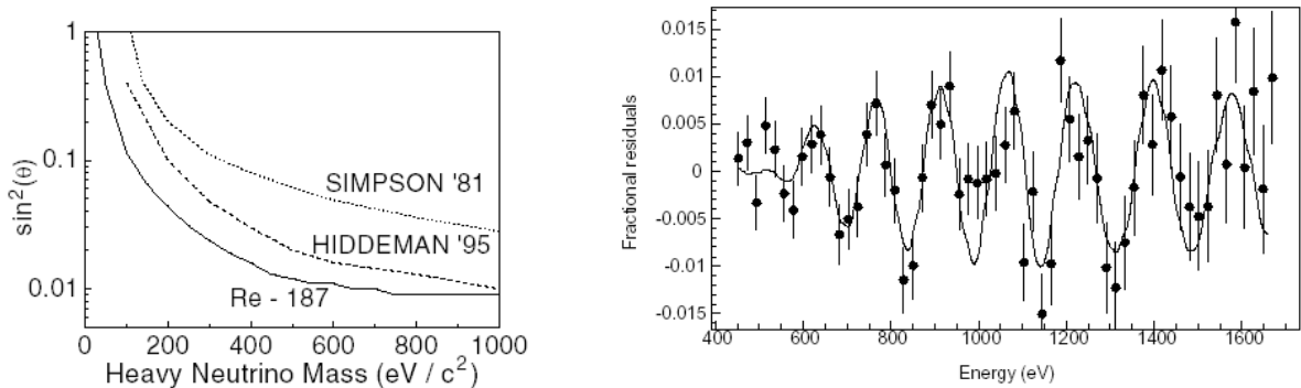
Figure 19: Heavy sterile mass exclusion plot of MANU [109] (left). BEFS in the MANU spectrum [110] (right).
