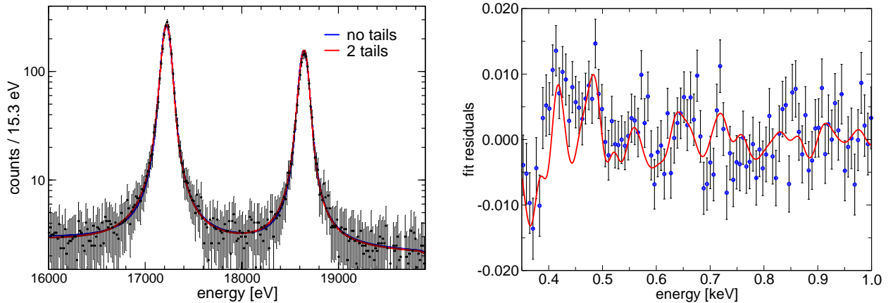
Figure 22: Escape peaks due to the exposure of \text{AgReO}_4 microcalorimeters to a ^{44}\text{Ti} source [120] (left) BEFS in the MIBETA final spectrum [106] (right).
