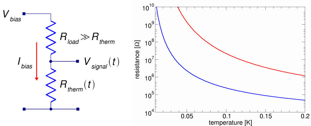
Figure 10: Constant current biasing of thermistors (left). Temperature dependence of the thermistor resistivity for a T_0 of 3 K (blue) and 10 K (red) (right).
