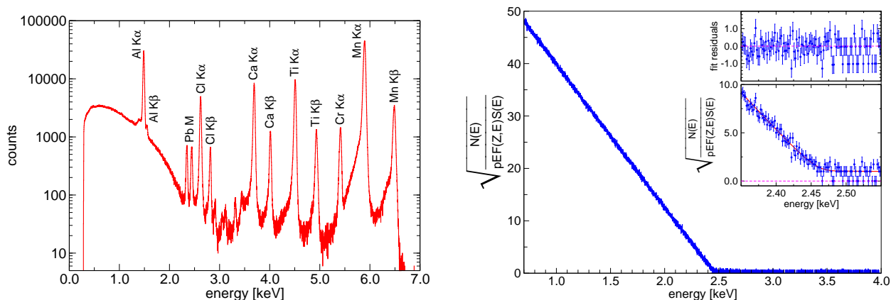
Figure 21: Final MIBETA calibration spectrum (left). Kurie plot of the final MIBETA data (right).
