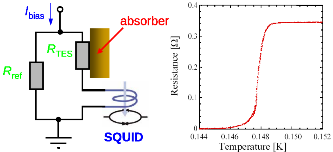
Figure 11: Constant current biasing of a TES (left). Temperature dependence of the TES resistivity at T_c (right)
