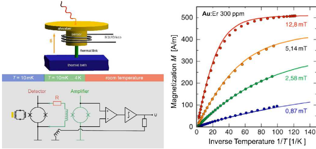
Figure 12: Read-out of a paramagnetic sensor (left). Temperature dependence of the sensor magnetization (right)
