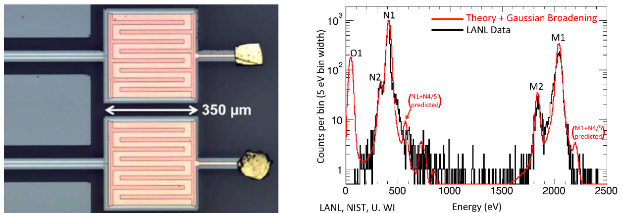
Figure 32: NuMECS TES detectors (left) and the latest spectrum measured from NuMECS (right), see text (from [157]).
