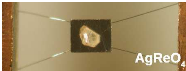
Figure 20: One of the MIBETA microcalorimeters with \text{AgReO}_4 .
