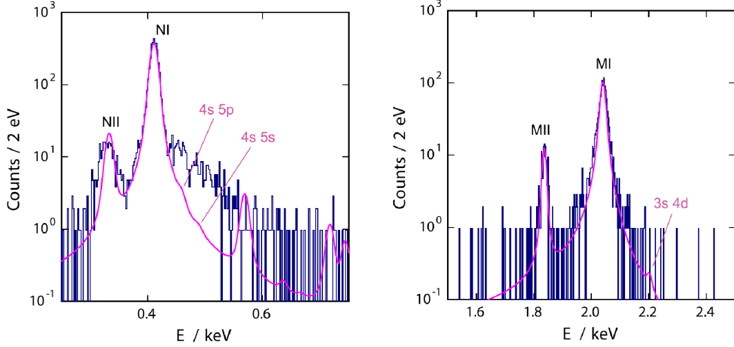
Figure 30: Latest measured spectrum from ECHO, see text (from [148]).
