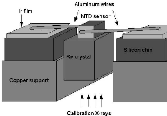
Figure 17: The MANU experiment detector (from [108]).
