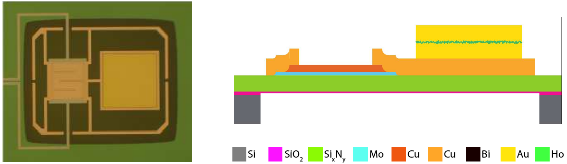
Figure 31: HOLMES TES pixel
