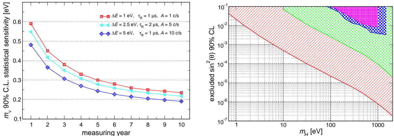
Figure 23: Statistical sensitivity of MARE final experiment. Curves are calculated for the deployment of 10000 pixels per year for the first 5 years (left). Statistical sensitivity to the emission of heavy neutrinos with mass m_H . From lower to upper curve: Monte Carlo simulation with N_{ev} = 10^{14} , f_{pp} = 10^{-6} and \Delta E = 1.5 eV; Monte Carlo simulation with N_{ev} = 8 \times 10^9 , f_{pp} = 10^{-5} and \Delta E = 15 eV; MIBETA experiment (unpublished); MANU experiment [109] (right).
