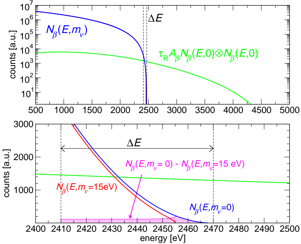
Figure 8: Effects of pile-up on the experimental energy spectrum of ^{187}\text{Re} beta decay. Higher panel: beta spectrum compared with pile-up spectrum. Lower panel: zoom around the end-point, with a comparison between 0 and finite neutrino mass beta spectra
