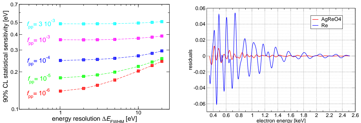
Figure 16: Monte Carlo computed statistical sensitivity of a ^{187}\text{Re} decay calorimetric measurement for different experimental configurations and for N_{ev} = 10^{14} (left). BEFS ripple prediction for metallic rhenium and for \text{AgReO}_4 for an infinite instrumental resolution (right).
