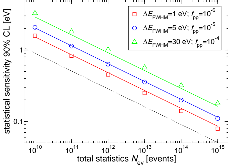
Figure 9: Statistical neutrino mass sensitivity for calorimetric measurements of the ^{187}\text{Re} beta decay. Lines are obtained from (34) according to [49]. Symbols are obtained with Monte Carlo simulations (§ 6.3).
