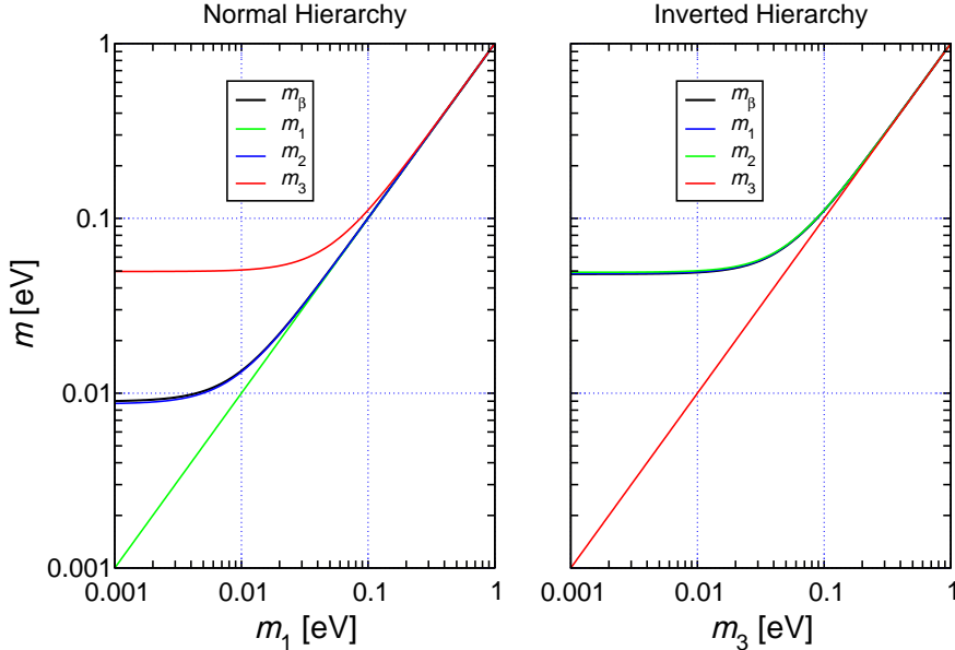
Figure 3: Effective electron neutrino mass m_\beta as a function of the lightest mass in both NH and IH mass schemes. The values of all three mass states are also plotted for comparison.
