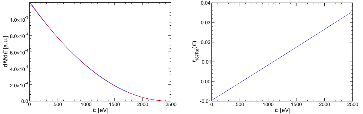
Figure 15: Theoretical shape of the ^{187}\text{Re} beta decay spectrum (left). Deviation of the ^{187}\text{Re} spectrum from a simple quadratic form (right).
