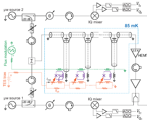
Figure 14: Circuit schematic for a two channel microwave multiplexed read out of a TES array (From [84]).
