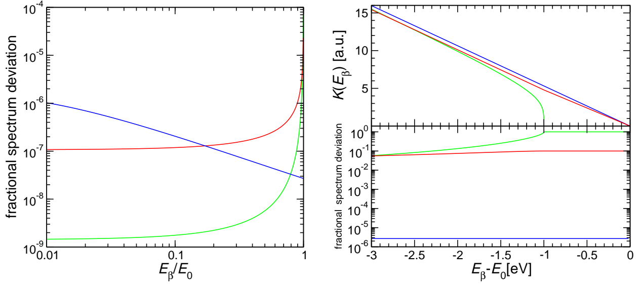
Figure 7: These plots compare the effect of a final excited state ( V_1 = 1 eV and \omega_1 = 0.1 eV) on the beta spectrum as measured with a calorimeter (blue) and with a spectrometer (red), and the effect of m_{\nu_e}^2 = 1 eV (green). The fractional spectrum deviation is the quantity 1 - N^*(E_\beta)/N(E_\beta) , where N^*(E_\beta) and N(E_\beta) are respectively the observed beta spectra with and without excited final state.
