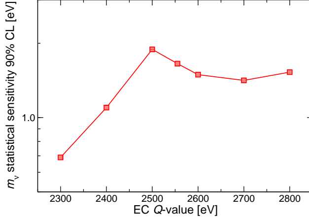
Figure 26: Monte Carlo computed statistical sensitivity as function of Q for N_{ev} = 3 \times 10^{13} and with f_{pp} = 3 \times 10^{-4} , \Delta E_{FWHM} = 1 eV, and no background.
