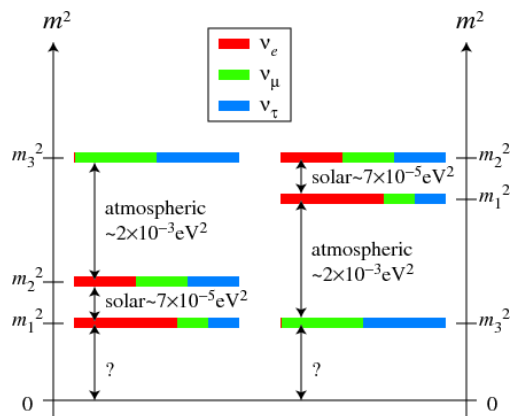
Figure 1: In a three-neutrino scheme, the oscillation parameters measured by the various experiments paint two possible scenarios regarding the neutrino mass ordering: Normal Hierarchy (left) and Inverted Hierarchy (right). The absolute scale is not accessible by presently available data.
