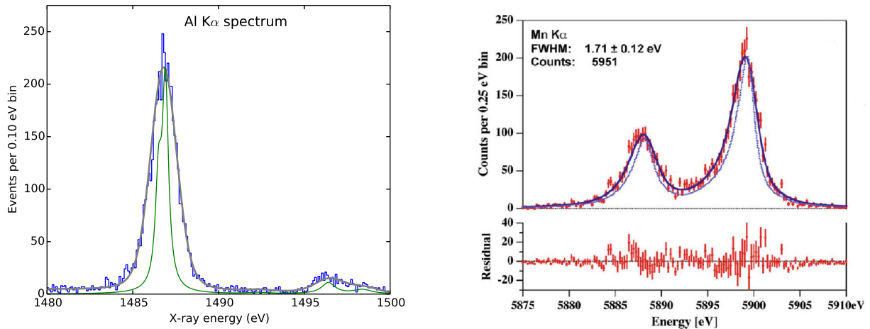
Figure 13: Energy resolutions achieved with a TES ( \Delta E_{\text{FWHM}} = 1.5 \text{ eV} , courtesy of NIST) (left) and with an MMC [80] (right).
