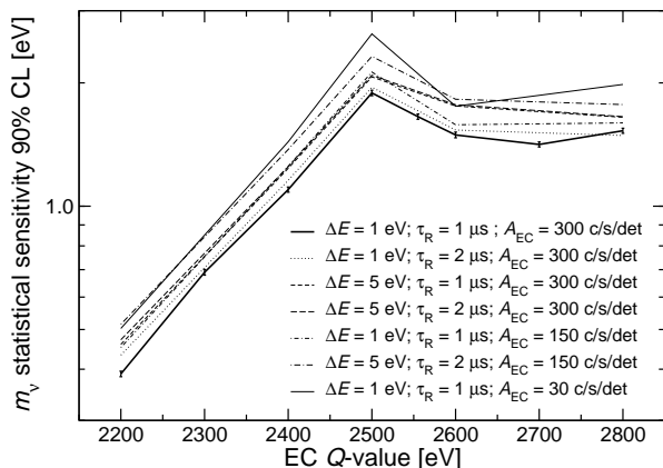
Fig. 8 Monte Carlo estimates of the effect on HOLMES baseline statistical sensitivity of different deviations from the baseline configuration and planned performance.
