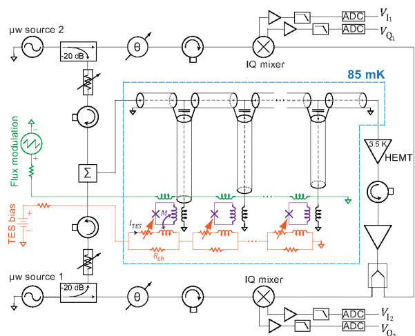
Fig. 7 Circuit schematic for a two channel microwave multiplexed read out of a TES array (from [31]).
