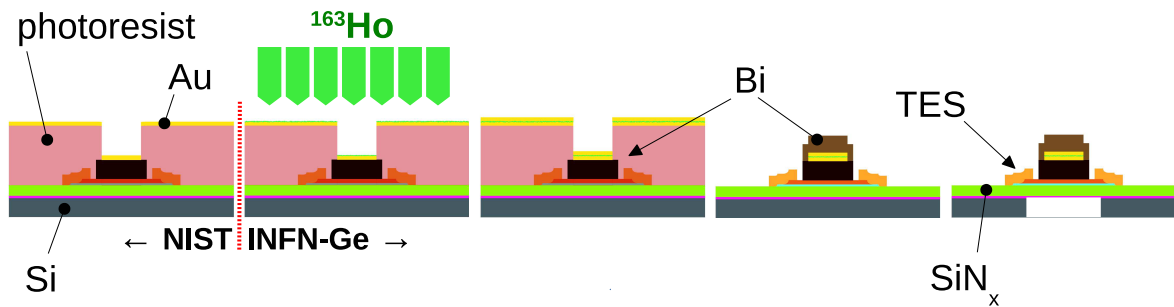
Fig. 6 The two step TES fabrication process.
